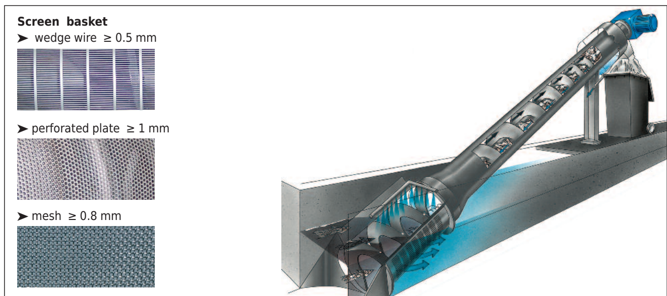
Schematic drawing of a ROTAMAT® Micro Strainer Ro 9
